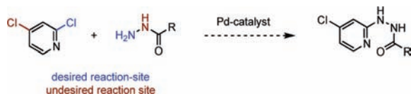
Scheme 2. Desired Regioselectivity
